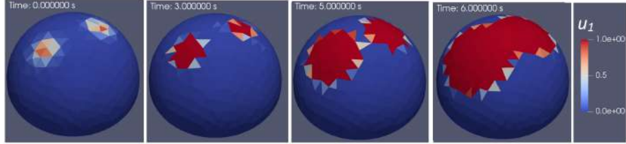
Figure 1: Numerical study of a nonlinear mixed-dimensional system (fully-discrete): two biofilm patches that stick to the surface of a sphere interact and grow by consuming nutrients ( N_2 and O_2 ) from the interior.
